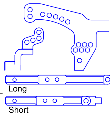
Shock Mount & Camber Link
