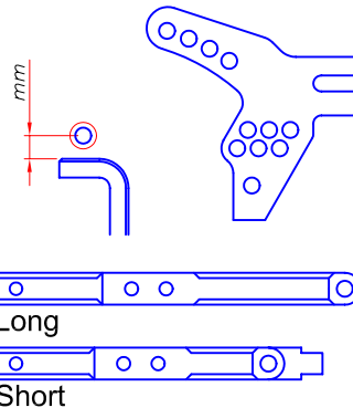
Shock Mount & Camber Link
